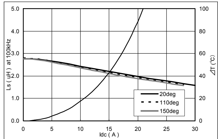
CDMC10D50T150NP-4R3M
